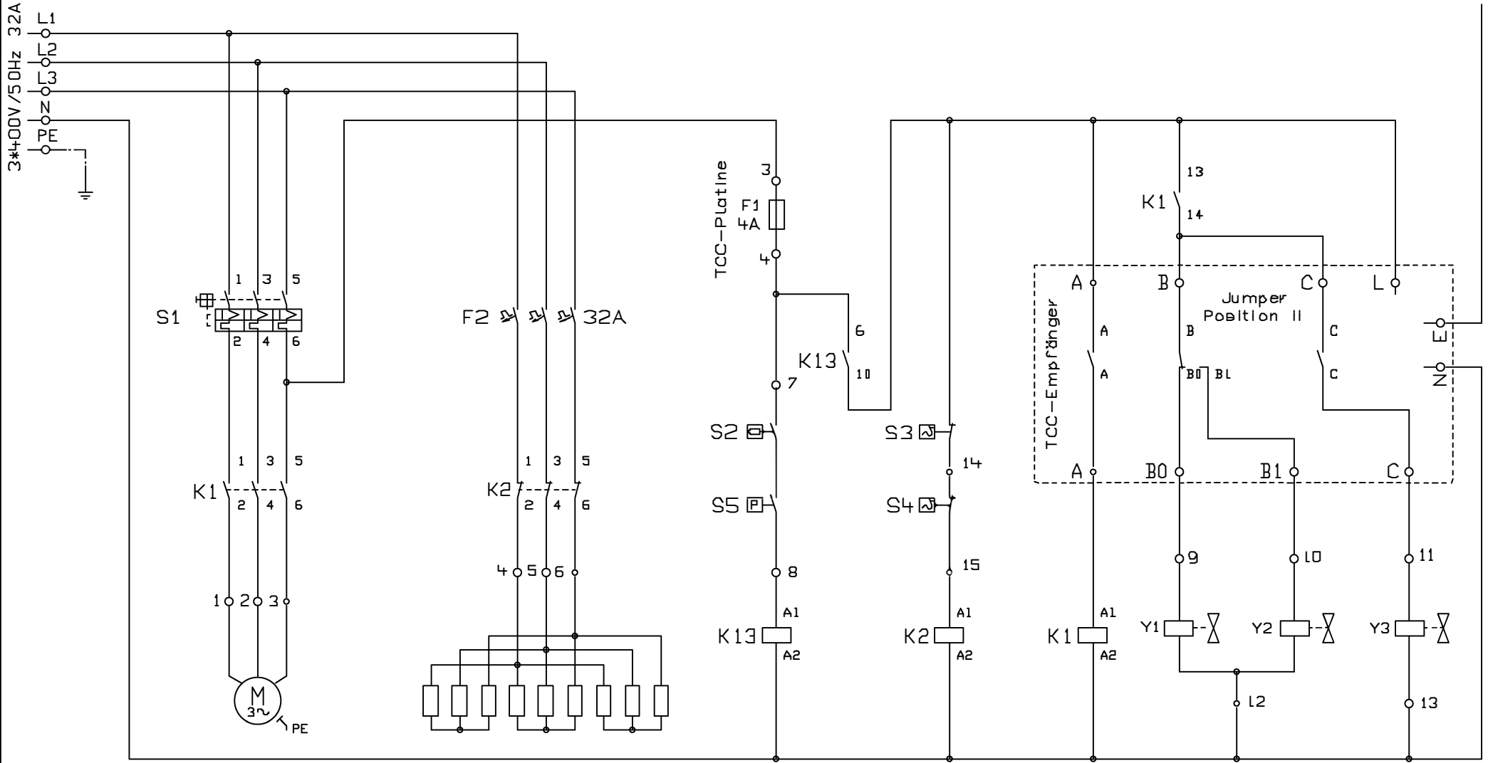
HD-Pumpe
