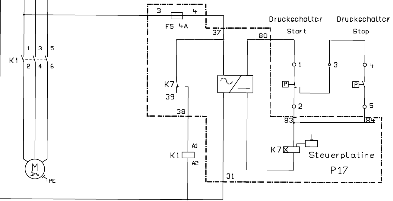
Motor-Pumpe
